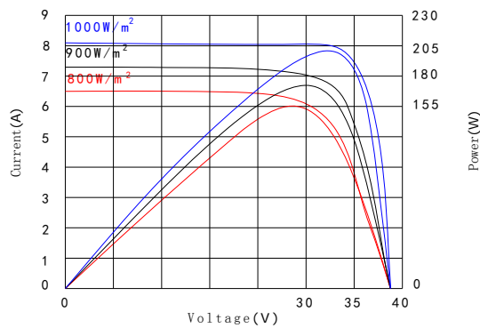
Electrical Performance cell temperature: 25°C
